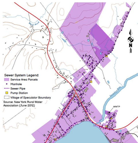
Figure 18: Village of Speculator Sewer System
